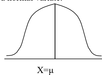
Fig: Normal probability curve
